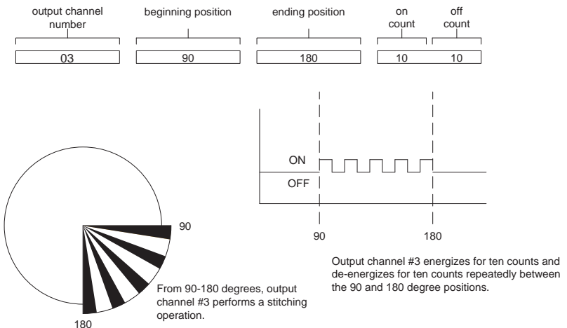
Figure 4-3 Positions for a Stitching Operation
